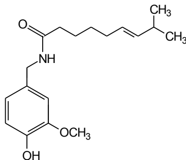
Dihydrocapsaicin
