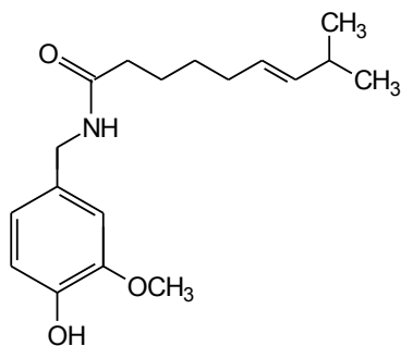
Capsaicin
